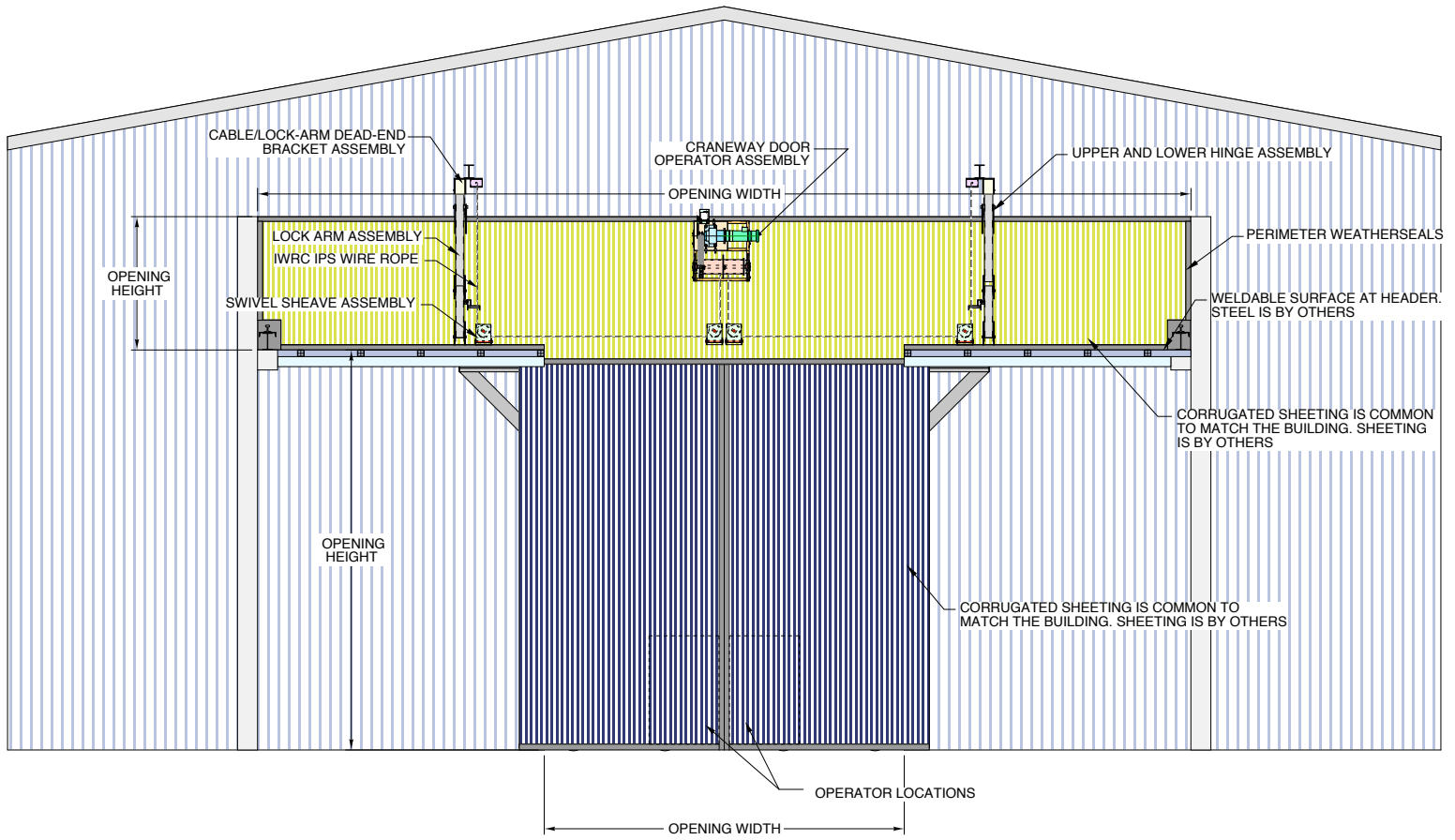
INTERIOR ELEVATION VIEW @ THE C-SERIES CRANEWAY AND H-SERIES BOTTOM ROLLING LOAD DOOR SYSTEM
