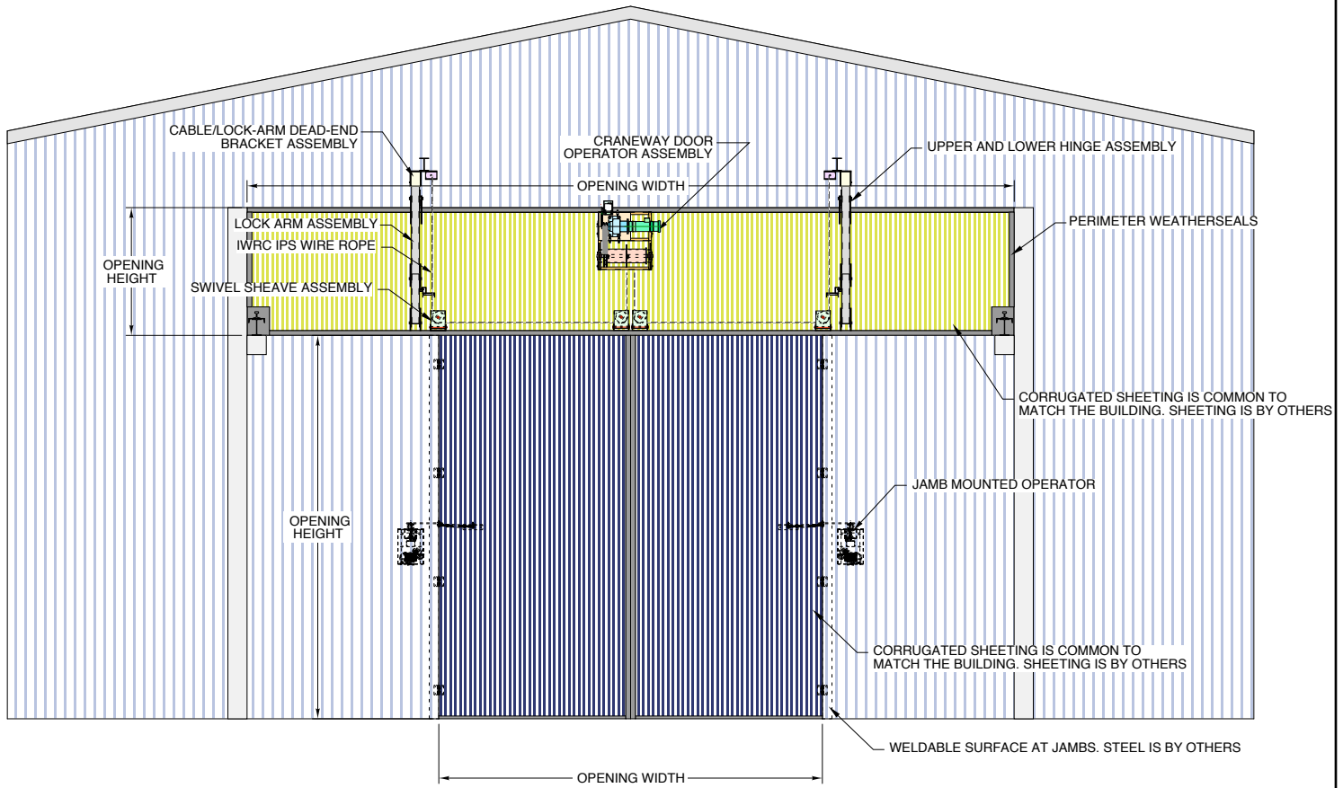
INTERIOR ELEVATION VIEW @ THE C-SERIES CRANEWAY AND S-SERIES SWING LOAD DOOR SYSTEM
