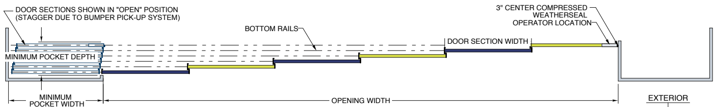
X X X PLAN VIEW SHOWING DOOR SECTIONS NORTHERN STACK DESIGN SHOWN
