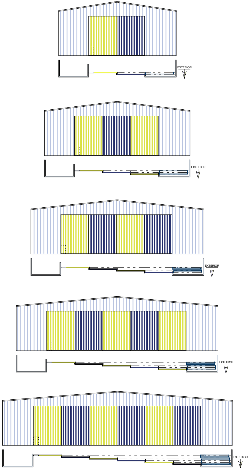
EXTERIOR ELEVATION & PLAN VIEWS @ THE H-SERIES MODEL HU200-HU600 HANGAR DOORS
